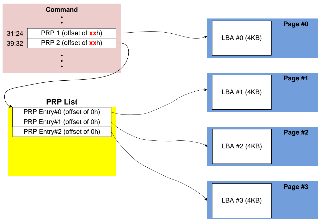
Figure 211: PRP List Describing Data to Compare
