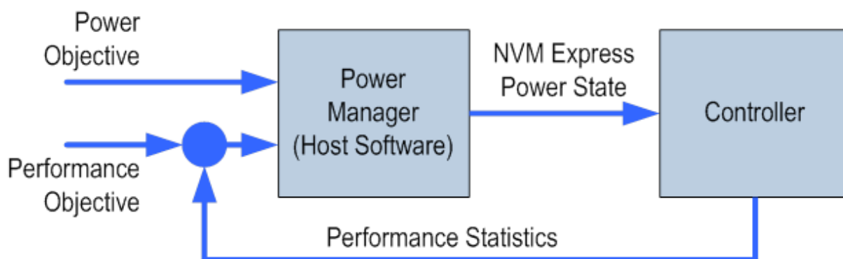
Figure 218: Dynamic Power Management
