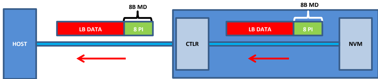
Figure 216: Read Command Protection Information Processing
